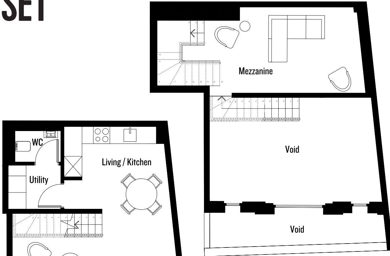
MEZZANINE FLOOR
